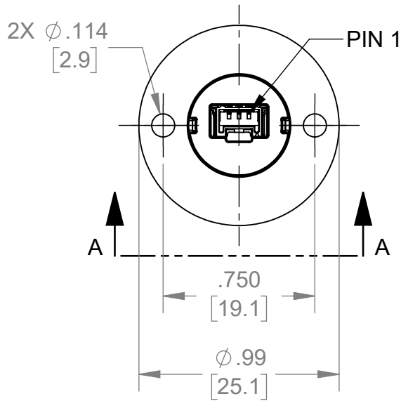
.750" BOLT CIRCLE
