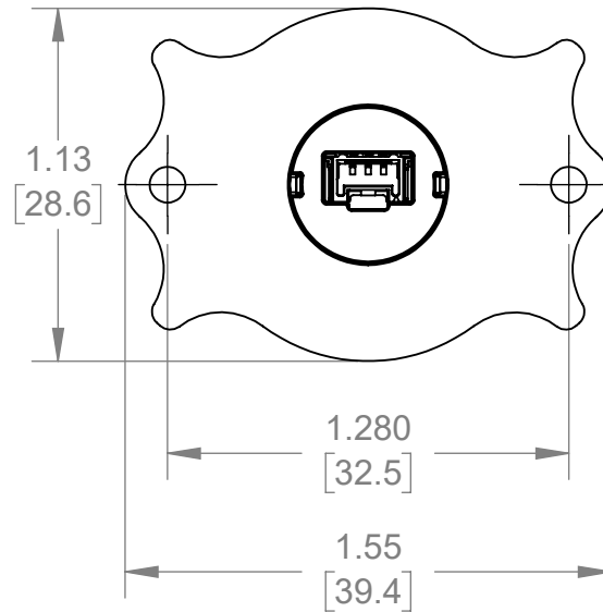
1.280" BOLT CIRCLE
