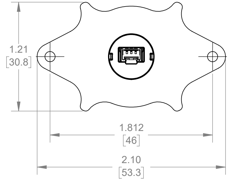
1.812" BOLT CIRCLE
